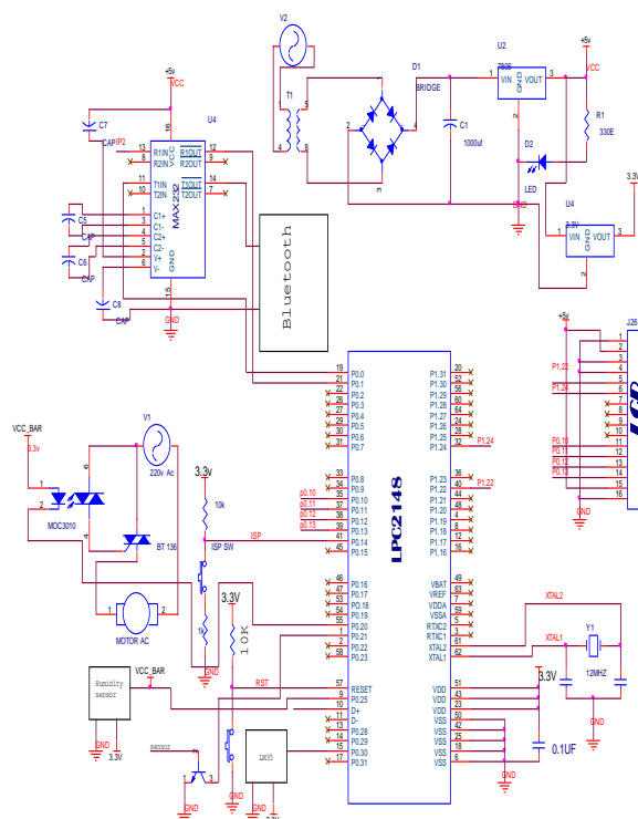
Fig 2: Schematic Diagram.
