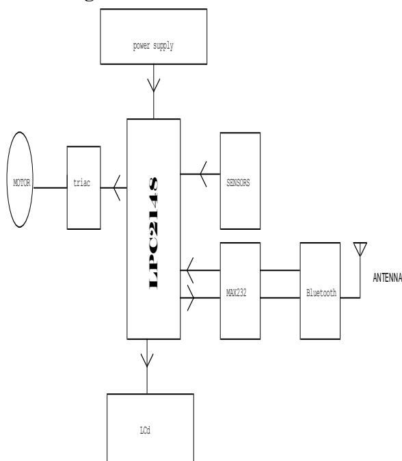
Fig 1: Block Diagram.
